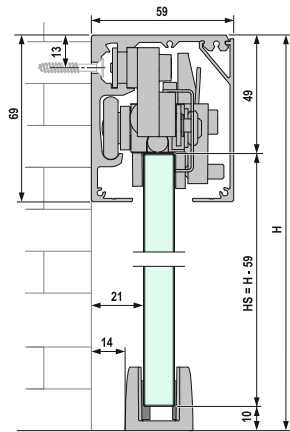
Wandmontage
