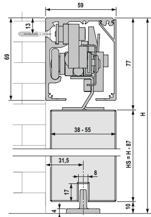
Wandmontage
